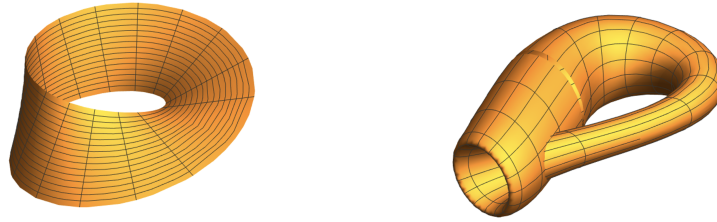
Figure 9. Two unorientable surfaces: the Möbius strip on the left, and the Klein bottle on the right.
