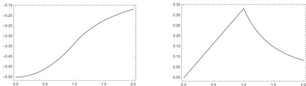
Figure 17. The plot of \Phi = -\psi/4\pi G on the left, with the radius R = 1 the cross over point. This is more apparent in the gravitational field g = -\Phi' shown on the right.
